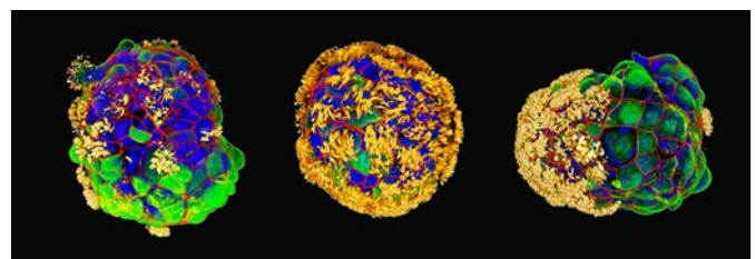
Anthrobot
