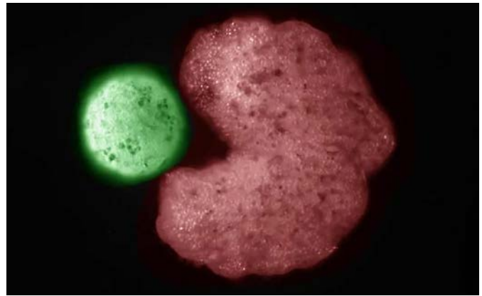
Xenobot
