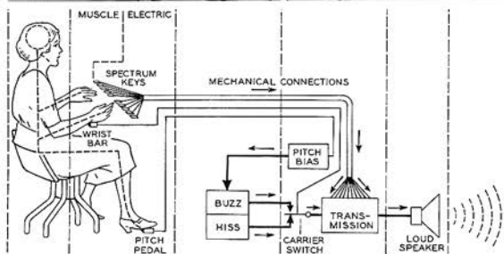
Fig. 8—Schematic circuit of the voder.
